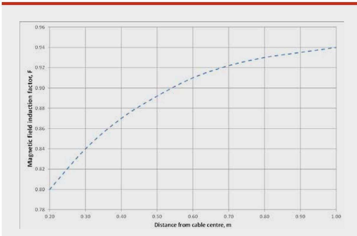
FIGURE 6.4 NORMALISED INDUCTION FACTOR TO CALCULATE THE EQUIVALENT UNIFORM FIELD AFTER BRACKEN AND DAWSON (2004)
