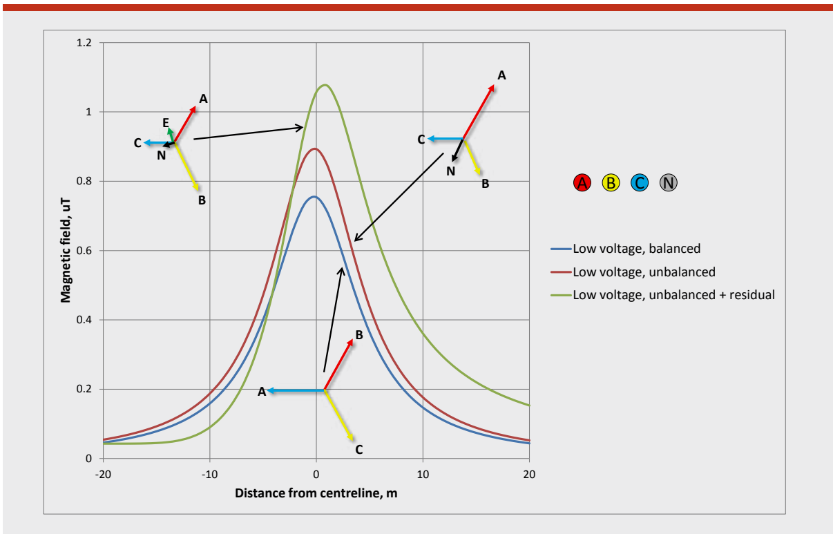
FIGURE 9.6 MAGNETIC FIELD PROFILES ASSOCIATED WITH LOW VOLTAGE CONSTRUCTION
